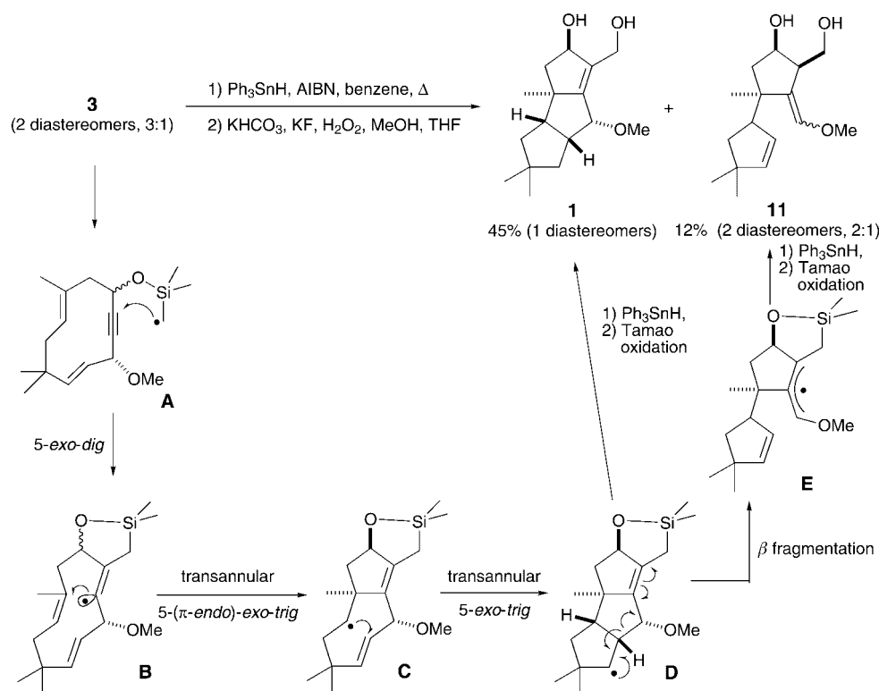
Scheme 4. Radical transannular cascade.
