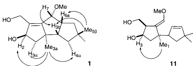
Scheme 5. NOE measurements for stereochemical assignments of 1 and 11 .
