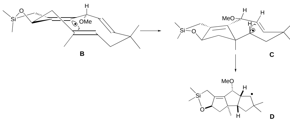
Scheme 6. Model for stereoselectivity.
